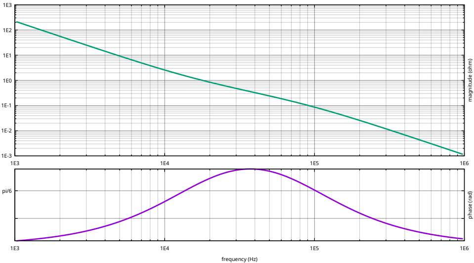
Loop Gain vs. Frequency
